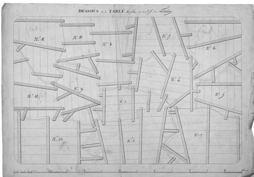
Figure 4. Below the table of the plan-relief of Toulon with bars of assembly, 1795, © Paris, Musée des Plans-Reliefs.
